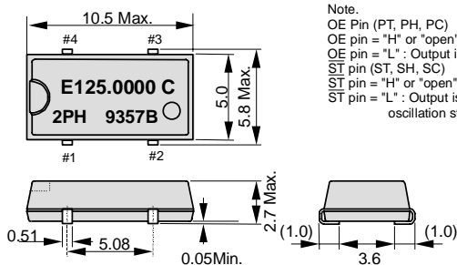
Pin map
