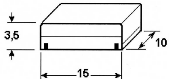
(unit: mm)
