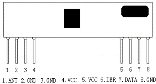
Figure1 CY07-V1.1Shape & Pins
