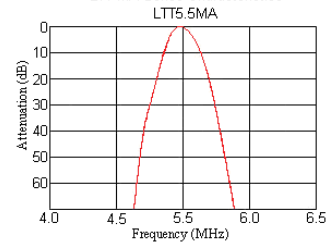
LTT MA Series Characteristics
