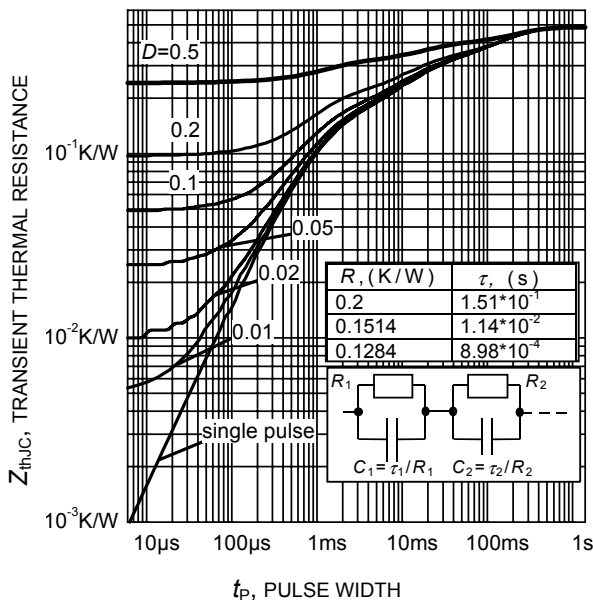
Figure 19. IGBT transient thermal resistance ( D = t_p / T )
