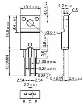
TO-220F
