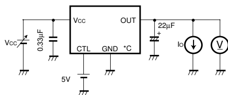
Fig.1 Measurement circuit for output voltage, input stability, load regulation, and temperature coefficient of output voltage
