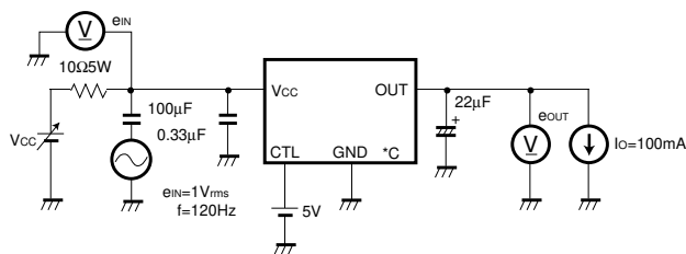
Fig.2 Measurement circuit for ripple rejection ratio
