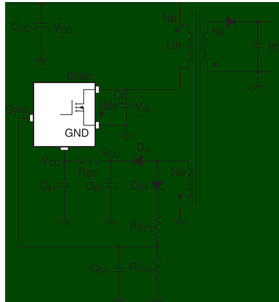
Figure 6. Synchronization Circuit
