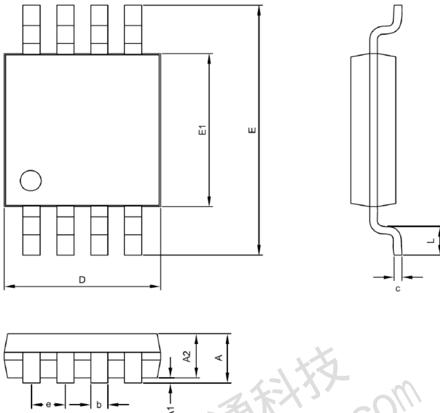
MSOP-8 Package
