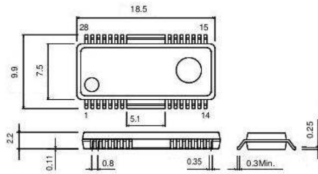
HSOP28 / HSOP-M28
