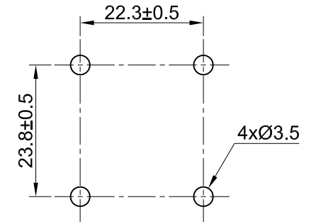
PCB/MOUNTING LAYOUT
