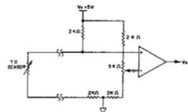
Figure 3 Adjustable Point (Comparator) Circuit
