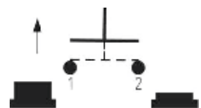
4T DPST OFF - ON × 2
