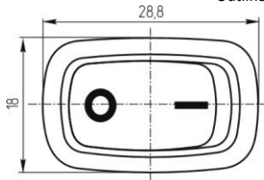
Outline Drawing
