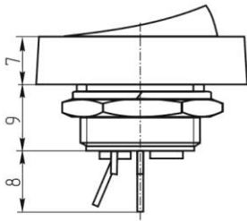
Mounting
