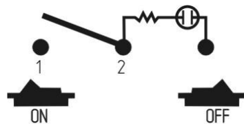
3P SPST (ILLUMINATED)
