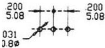
Mounting
