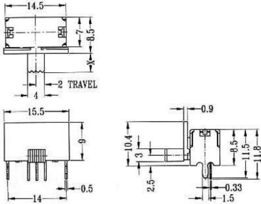
Outline Drawing
