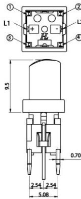
Outline Drawing
