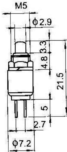
Outline Drawing
