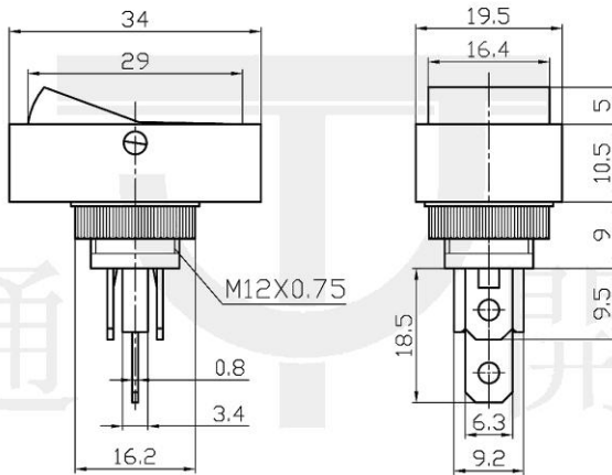
Mounting
