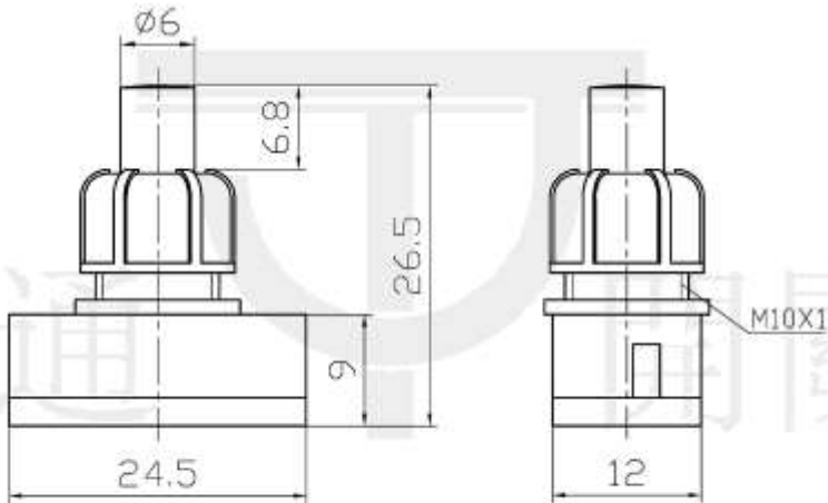
Outline Drawing
