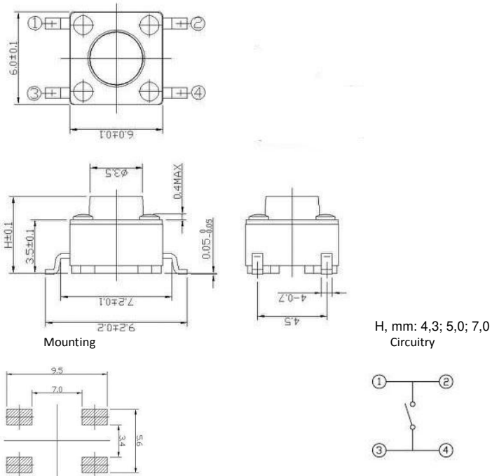
Outline Drawing
