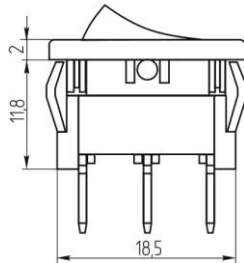
Mounting
