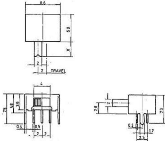
Outline Drawing
