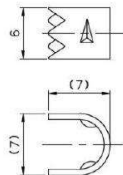
Cable Clamp
