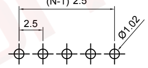
Recommend PCB layout (Tolerance:±0.05)
